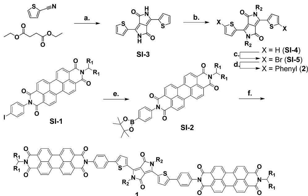
Scheme 1 Synthesis of molecules 1–2. a–a (a) t -Amyl alcohol, KOtBu, 120 °C, 34% (b) DMF, K 2 CO 3 , 1-bromodecane, 120 °C, 85% (c) DCM, NBS, RT, 59%, (d) toluene, EtOH, H 2 O, K 2 CO 3 , phenylboronic acid, Pd(PPh 3 ) 4 , 60 °C, 95%, (e) DMF, bis(pinacolato)diboron, KOAc, Pd(dppf)Cl 2 , 100 °C, 98%, (f) toluene, EtOH, H 2 O, K 2 CO 3 , SI-5, Pd(PPh 3 ) 4 , 65 °C, 64%.
