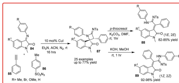
Scheme 42 Copper(I) catalyzed one-pot, three-component diastereoselective synthesis of 3-spiroazetidiniimine-2-oxindoles.
