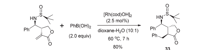
Scheme 15 Rhodium-catalyzed arylation of anti -isomer to introduce another chiral center.
