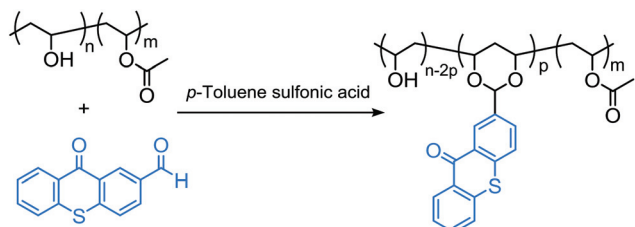
Scheme 20 Synthesis of poly(vinyl alcohol) thioxanthone macrophotoinitiator.
