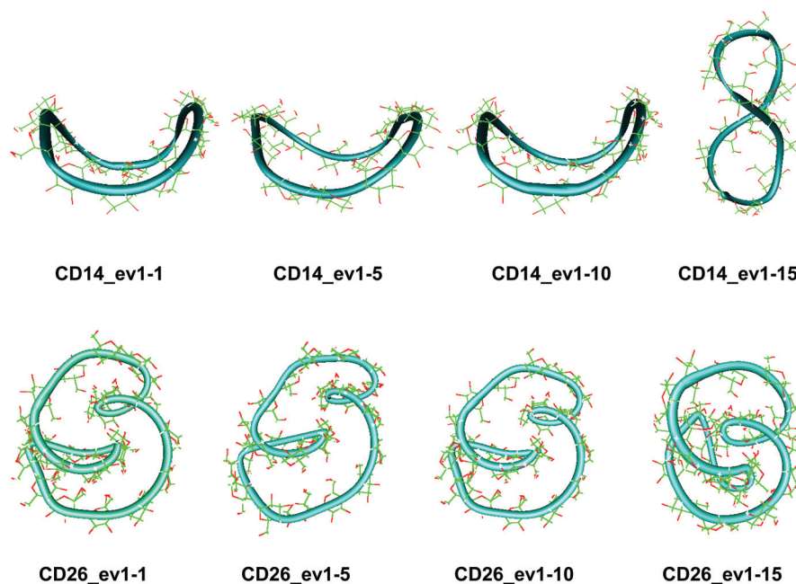
Fig. 4 Snapshots (with sequential numbers 1, 5, 10 and 15) of the first animated eigenvector ( ev1 ) having the largest contribution to the total variance of the atomic fluctuations: (a) CD14 (PCA, 60.0 ns); (b) CD26 (PCA, 100.0 ns).
