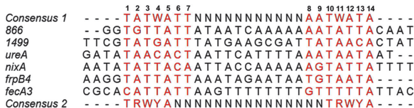
Fig. 5 Alignment of the HpNikR binding sites from select promoters. The two parts of the consensus sequence are bolded, in red, and numbered according to Evans et al. for the aligned sequences. 62 Consensus 1 and Consensus 2 represent the DNA recognition sites proposed by Delany et al. 28 and Stoof et al. , 29 respectively. N represents any nucleotide and W represents either an A or T nucleotide. Clustal Omega was used to align the promoters and generate the image.
