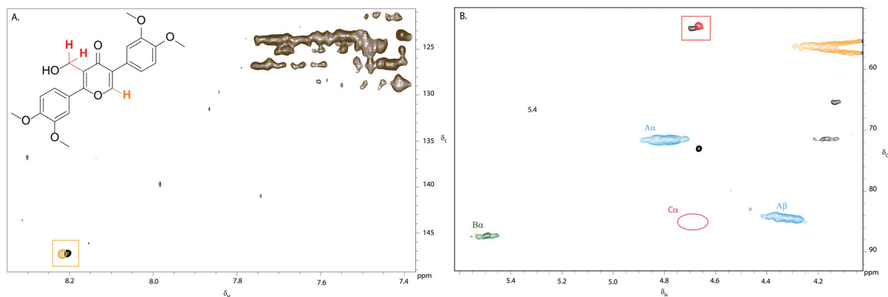
Fig. 5 Overlay of partial 2D HSQC NMR spectra of (i) Kraft lignin after treatment with 0.75 weight equivalents of DDQ and (ii) of an authentic sample of pyran-4-one 5 : (A) aromatic region ( \delta_{\text{C}}/\delta_{\text{H}} 120–150/7.4–8.4) and (B) aliphatic region ( \delta_{\text{C}}/\delta_{\text{H}} 50–90/4.0–5.6). The close proximity of the aromatic and methylene cross peaks in 5 with new cross peaks present in the DDQ-treated lignin spectrum are shown in orange and red boxes respectively. Contours are colour coded according to the linkage they are assigned to (see Fig. 2 legend).
