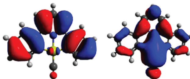
Fig. 2 HOMO (left) and LUMO (right) of [(C ^ N ^ C)Au(CO)] + as simulated by DFT.
