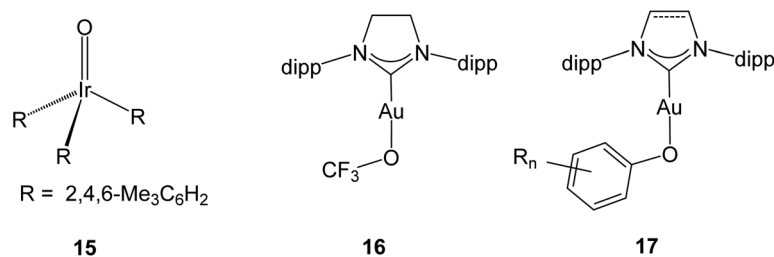
Scheme 10 Examples of metal oxo and gold(I) alkoxide complexes (dipp = 2,6-Pr 2 C 6 H 3 ).
