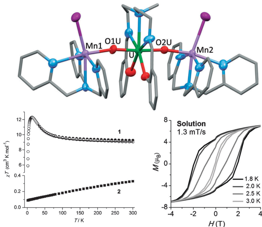
Fig. 17 (top) Molecular structure of \{[M(\text{TPA})][\text{UO}_2(\text{Mesalدين})][M(\text{TPA})]\} ( M = \text{Mn} (\text{Mn}_2\text{U}), \text{Cd} (\text{Cd}_2\text{U}) ) with hydrogen atoms omitted for clarity; (bottom left) Susceptibility temperature product as a function of temperature for \text{Mn}_2\text{U} (1) and \text{Cd}_2\text{U} (2), as well as their difference (open symbols), showing the effective ferromagnetic coupling between \text{U}^{\text{V}}\text{O}_2 and \text{Mn}^{\text{II}} . (bottom right) Magnetic hysteresis recorded on a pyridine solution of \text{Mn}_2\text{U} . Adapted with permission from ref. 54. Copyright 2014 Wiley-VCH.
