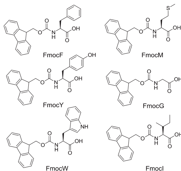
Fig. 1 Structures of the Fmoc amino acid LMWG.
