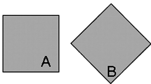
Fig. 15 Scheme for a chemical diode based on unidirectional propagation of chemical waves. A and B are the excitible media, i.e. , the glass plates with ferroin loaded on their surfaces. The waves propagate only from A to B and not vice versa .
