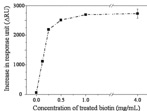
Fig. 2 Binding level of streptavidin on the dendrimer monolayer that had been biotinylated with various concentrations of succinimidyl \alpha -biotin.
