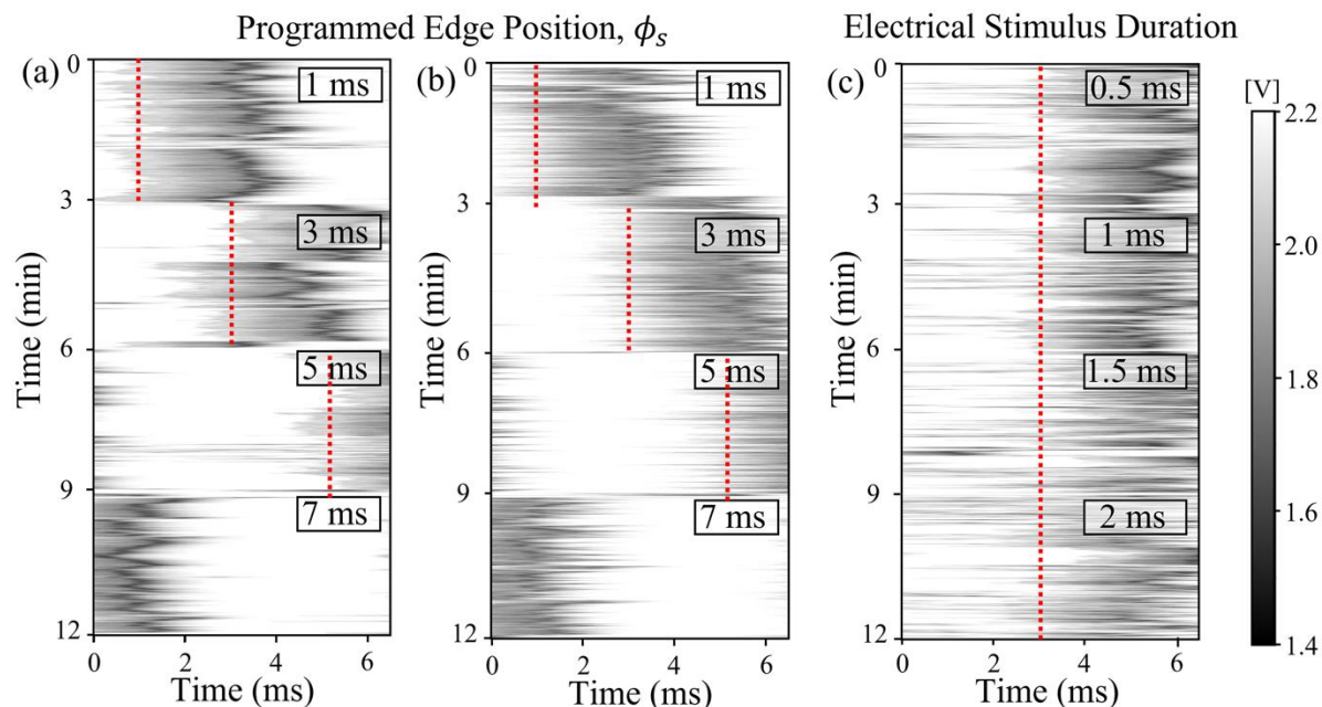
Figure 4: Examples for parameter sweeps to diagnose the droplet injection conditions: (a) The leading droplet edge position was changed from 1 to 7 ms in 2 ms steps, each being recorded for a 3 min run. The injected sample was NQO1. (b) as in (a), but the sample was phycocyanin. (c) The trigger duration was changed across 4 runs for NQO1 from 0.5 ms to 2 ms in steps of 0.5 ms. The greyscale color bar represents the amplitude of the droplet signal in volts and the red dotted line \phi_s .
