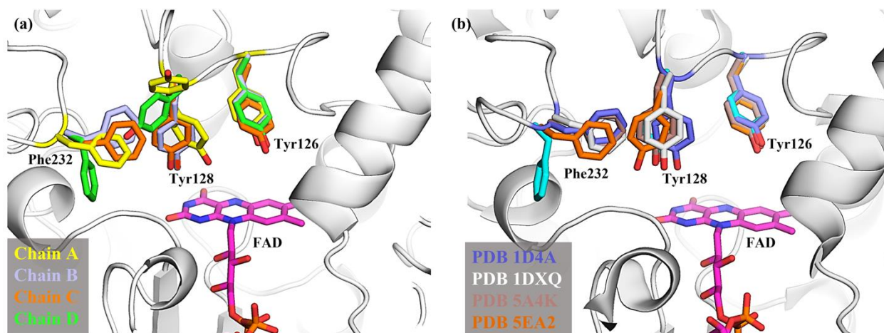
Figure 7: (a) Superimposition of the four monomers found in the asymmetric unit of the NQO1 structure determined at MFX. Residues Tyr126, Tyr128, and Phe232, key for NQO1 function, are represented as sticks. FAD is labeled accordingly and represented as pink sticks. (b) Superimposition of the four unliganded cryogenic structures of NQO1 (PDB 1D4A, 79 PDB 1DXQ, 79 PDB 5A4K 84 and PDB 5EA2 85 ). As in (a), the key residues and FAD molecule are highlighted.
