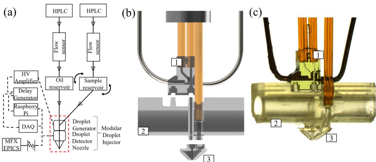
Figure 1: (a) Schematic set-up of the MDI and control hardware (not to scale) implemented at the MFX instrument. (b) Graphic of the three MDI components: 1) droplet generator, 2) droplet detector, 3) 3D-printed GDVN. Three silica capillaries (orange) deliver the oil/sample solutions and the GDVN sheathing gas. The NiCr wires (black) attached to the droplet generator allow electrical droplet stimulation. (c) A microscopic image of the MDI fully assembled with the same components as in (b).
