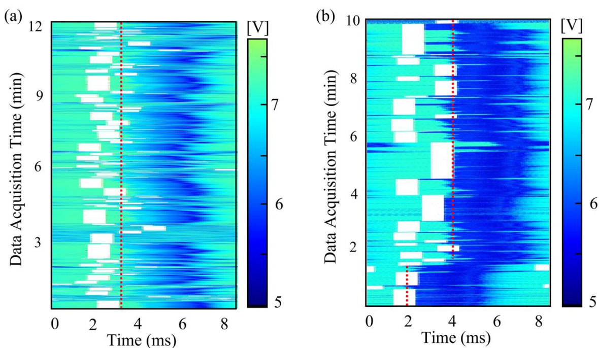
Figure 3: A characteristic waterfall plot depicting the background of oil in teal, the protein crystal-containing droplet in deep blue, the trigger signal in white, and \phi_s as a red dashed line for continuously triggered and locked-in droplets at 120Hz for (a) NQO1 and (b) phycocyanin during LW79 at the MFX instrument.
