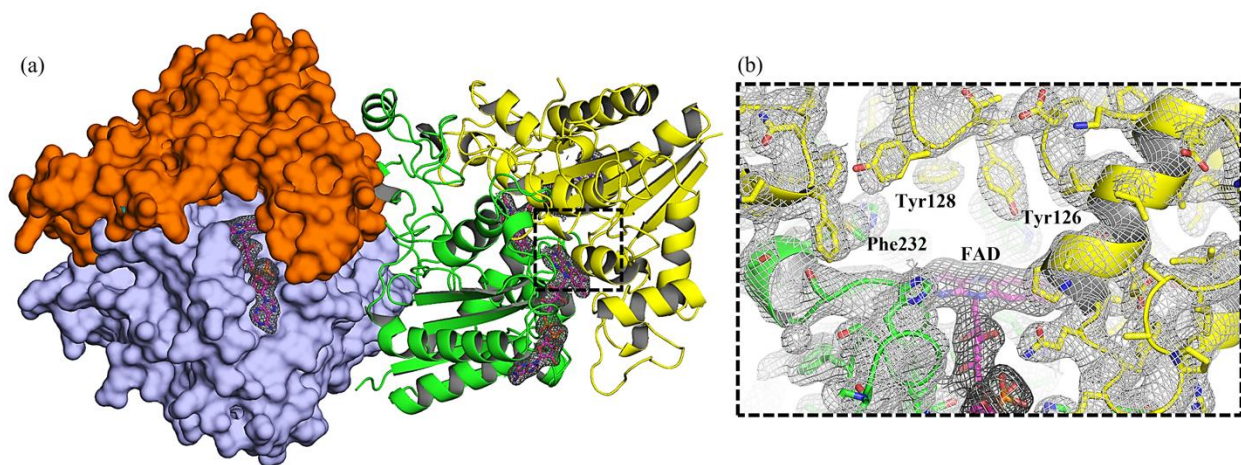
Figure 6: SFX structure of human NQO1 obtained at MFX. (a) The two dimers of NQO1 in the asymmetric unit are depicted. The individual monomers are highlighted in green, yellow, orange, and light blue. The cofactor FAD is shown as pink sticks. The catalytic site of one of the monomers is black-boxed. (b) Closer view of the catalytic site in (a). The electron 2mF_c-DF_o density maps at the catalytic site contoured at 1\sigma are shown. Residues Tyr126, Tyr128, and Phe232 which are key in the function of the enzyme are highlighted. Our results also suggest the presence of different conformational sub-states prior to NAD(P)H binding and consequent flavin reduction, thus supporting a conformational selection mechanism and providing structure-function information at high resolution.
