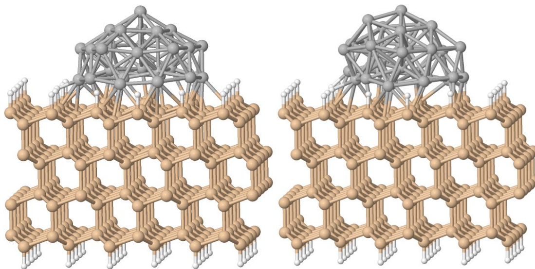
(a) \text{Ag}_{32}\text{Si}_{240}\text{H}_{52}
