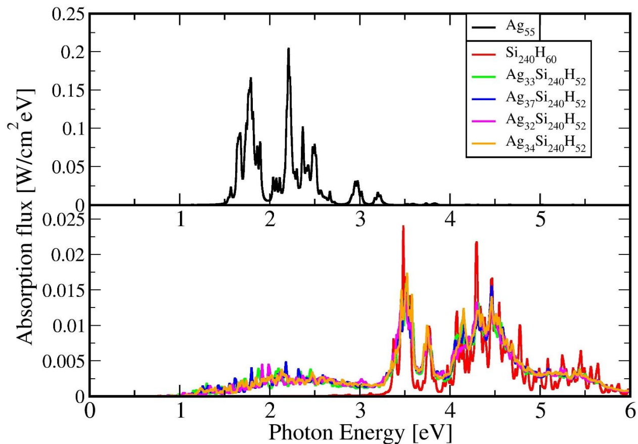
Fig 4 Light absorbance vs photon energy for the present \text{Ag}_n/\text{Si}(111) structures, pure Si surface and \text{Ag}_{55} using the HSE06 functional. In the upper panel the \text{Ag}_{55} values are shown and in the lower panel \text{Ag}_n/\text{Si}(111) structures and pure Si surface absorption values are shown.
