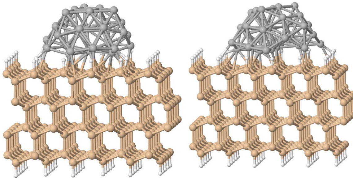
(c) \text{Ag}_{34}\text{Si}_{240}\text{H}_{52}
