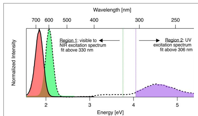
Figure 1: Prototypical excitation (dashed black line) and emission (solid black line) spectra for an \text{Ag}_\text{N} -DNA with single excitation and emission peaks. The emission spectrum is fitted to a single Gaussian (red shading) to determine peak emission energy E_\text{em} . The excitation spectrum is fitted to two single Gaussian peaks, one in the visible-NIR region at fitted peak energy E_\text{ex} (green shaded fit in Region 1) and one in the UV (purple shaded fit in Region 2). Signal between 306-330 nm is excluded due to stray light in some regions of the well plate from an imperfection in the plate reader. Stokes shift SS is calculated as SS = E_\text{ex} - E_\text{em} . The ratio of excitation peak areas in Regions 1 and 2 is defined as R_\text{UV/vis} = (\text{area of green Region 2 peak})/(\text{area of purple Region 1 peak}) . Figure S7 shows additional excitation spectra of samples excluded from analysis due to multiple peaks in excitation or emission spectra.
