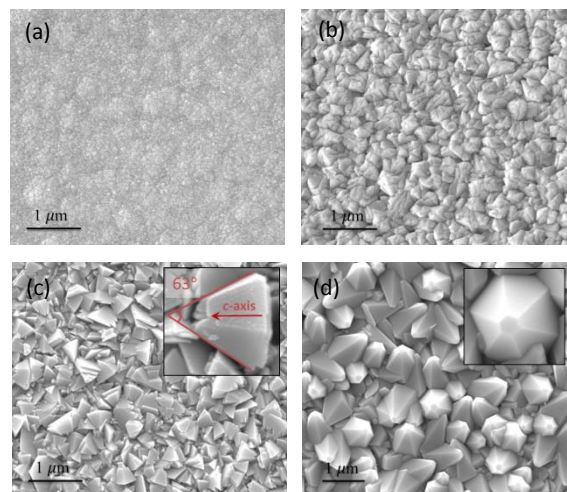
Figure 2 SEM images of ZnO films with (a) 0 mL, (b) 2 mL, (c) 4 mL and (d) 8 mL acetic-acid added in precursor solutions. The insets show higher magnification images for corresponding sample.
