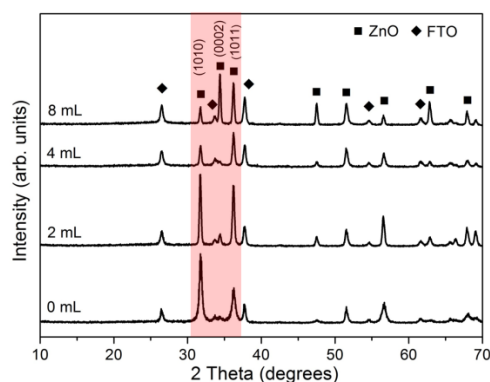
Figure 3 XRD patterns of ZnO films prepared with various acetic-acid contents in precursor solutions
