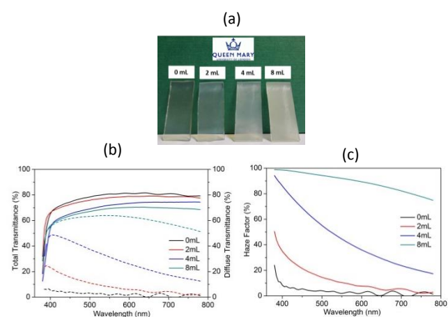
Figure 1 (a) Optical appearance, (b) UV-Vis total and diffuse transmittance and (c) haze factor spectra of ZnO films prepared with various acetic-acid contents in precursor solutions.
