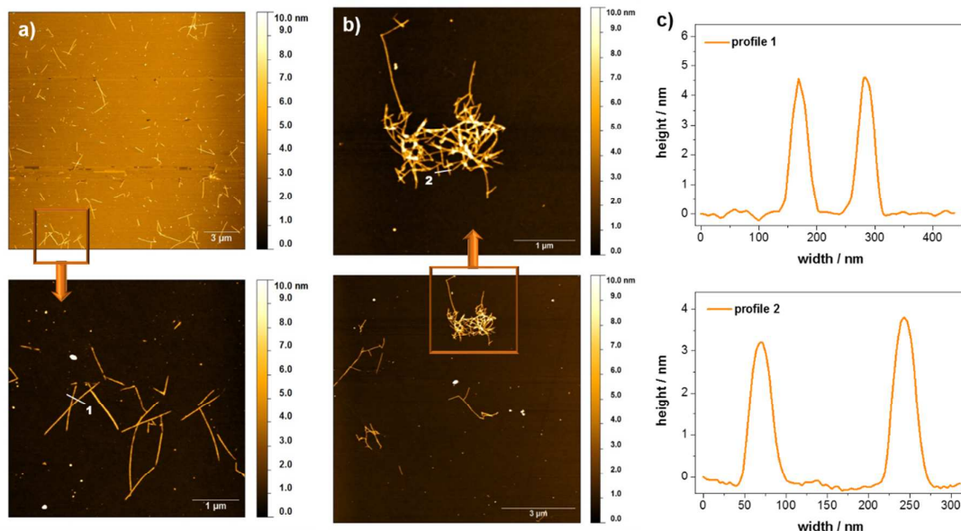
Figure 5: AFM images of 100-fold diluted hydrogel with 1.5 wt% 1 at a) pH 4 and b) pH 6 show rod like structures which assemble in a different manner. c) The height profiles 1 and 2 were marked within the zoom images. Silicon wafers were used as substrate.
