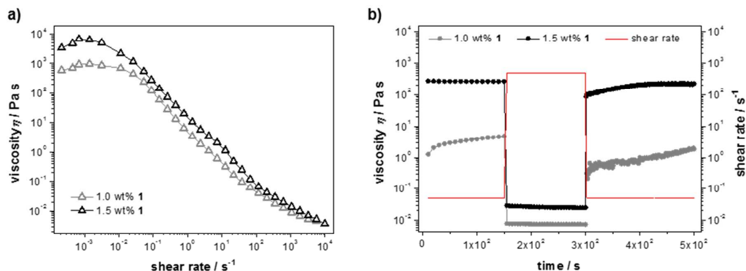
Figure 3: a) Steady shear rheological measurements reveal the response to increasing shear stress of solutions and hydrogels with 1.0 wt% and 1.5 wt% 1 . b) Step-rate measurements of samples with 1.0 wt% and 1.5 wt% 1 display the different recovery of the hydrogel network immediately after the breakdown due to a high magnitude shear rate.
