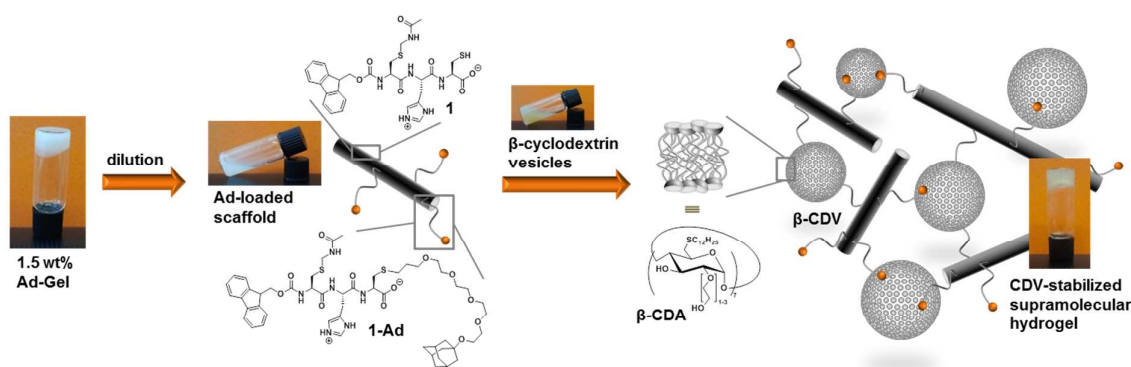
Figure 9: Formation of a stabilized supramolecular hydrogel of adamantane functionalized peptide scaffolds ( 1 : 1-Ad mixed 9 : 1 and cyclodextrin vesicles (CDV) of amphiphilic \beta -cyclodextrin host molecules ( \beta -CDA) via multivalent host-guest inclusion complexes at pH 6 (final concentrations are 0.75 wt% of 1 and 2 mM (0.6 wt%) CDV).
