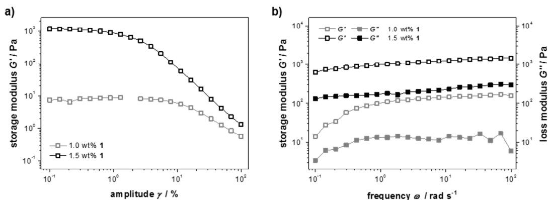
Figure 2: Oscillatory rheological measurements of solutions and hydrogels with 1.0 wt% and 1.5 wt% 1 . a) Storage modulus obtained from a strain-amplitude sweep performed at \omega = 10 \text{ rad s}^{-1} . b) Storage G' and loss G'' moduli obtained from a frequency sweep performed at \gamma = 0.5 \% .
