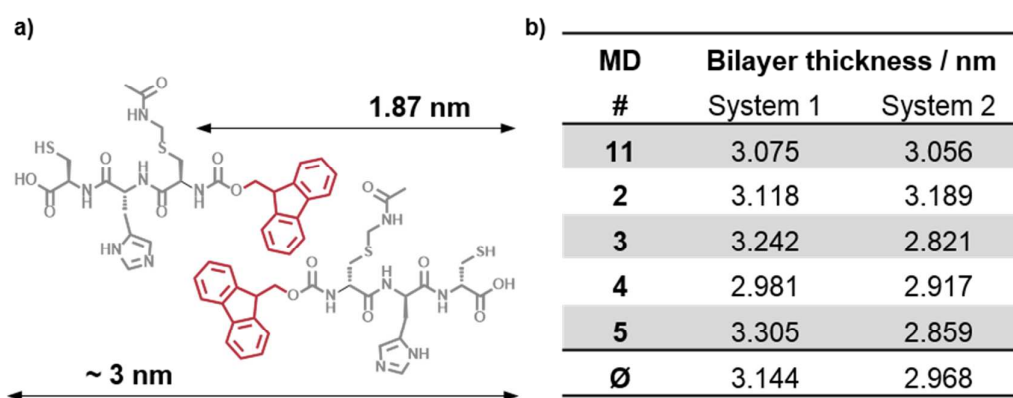
Figure 7: a) Schematic representation of the estimated membrane thickness from the calculated length of peptide 1 taking into account overlapping Fmoc-protection groups in the core of the bilayer. b) Average thickness of the bilayer models of peptide 1 and 2 , calculated from 100 evenly distributed snapshots for each independent 5 ns MD run.
