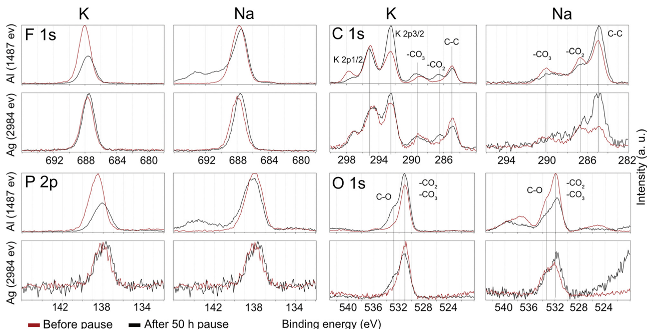
Fig. 4 F 1s, O 1s, P 2p, and C 1s XPS spectra of SEI formed in 1 M \text{KPF}_6 in EC:DEC and 1 M \text{NaPF}_6 in EC:DEC before and after a 50 h open circuit relaxation. The spectra were measured using two different photon energies of 1487 eV and 2984 eV from Al K\alpha and Ag L\alpha sources, respectively.
