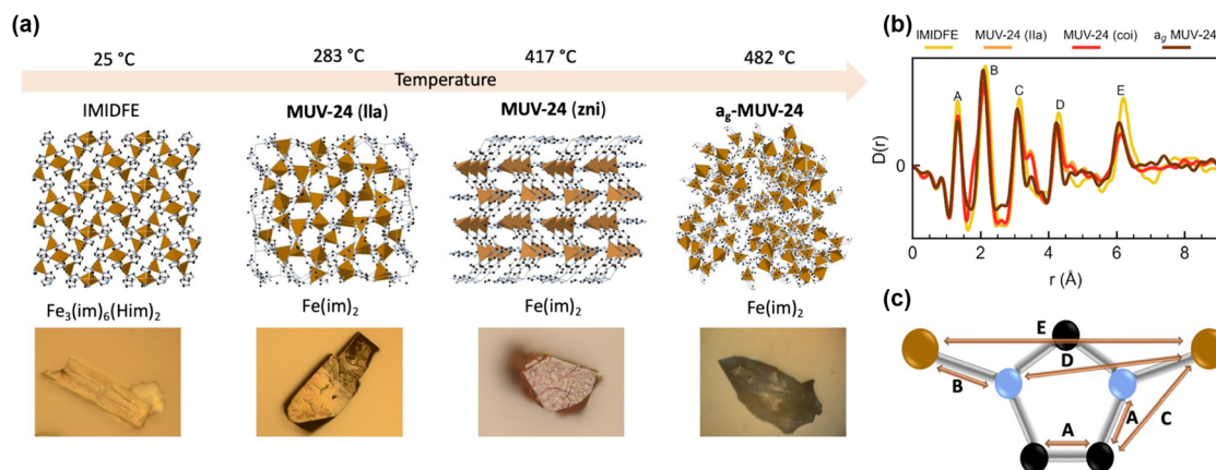
Fig. 25 (a) Temperature-driven phase evolution of IMIDFE to MUV-24 (IIa), MUV-24 (znl), and finally the amorphous glass a_g -MUV-24 (schematic), with the corresponding optical micrographs; vitrification is observed in the final material. (b) X-ray pair distribution functions, D(r) , for IMIDFE, MUV-24 (IIa), MUV-24 (coi), and a_g -MUV-24, showing retention of short-range order across phases. (c) Structural representation assigning short-range bonds/pair distances (Fe, brown; C, black; N, blue) to the labeled X-ray pair distribution peaks. Reproduced with permission from ref. 113, Copyright 2023, American Chemical Society.
