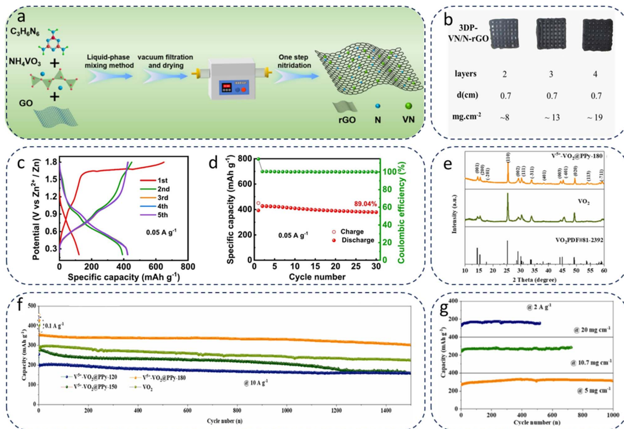
Fig. 8 (a) Schematic diagram of the preparation process of VN/N-rGO. (b) Photographs of 3DP-VN/N-rGO electrodes with different layers and varying mass loadings. (c) Discharge-charge curves and (d) cycling performance of the 3DP-VN/N-rGO electrode at 0.05 A g -1 . Reproduced from ref. 19 with permission from Elsevier, copyright 2025. (e) The XRD patterns of V 5+ -VO 2 @PPy and VO 2 materials. (f) The long-term cycle performance of four batteries at 10 A g -1 (Zn//V 5+ -VO 2 @PPy-120 150 180 and Zn//VO 2 ). (g) Cycle performance at 2 A g -1 based on various mass-loadings: 5, 10.7 and 20 mg cm -2 . Reproduced from ref. 15 with permission from Elsevier, copyright 2023.
