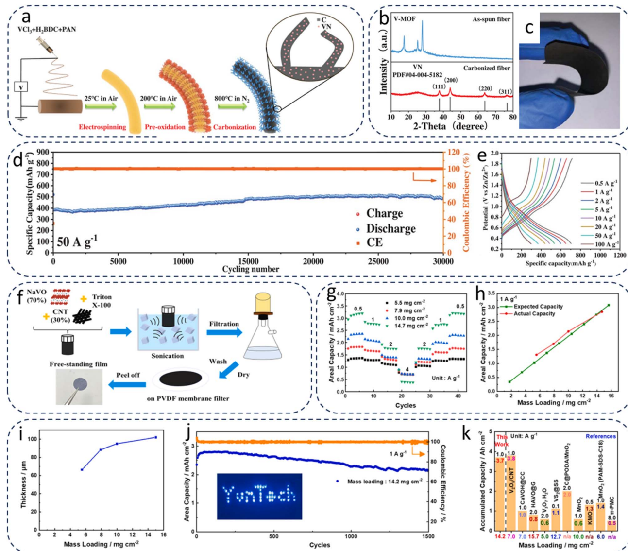
Fig. 11 (a) Schematic illustration of the synthesis procedures for the 3D self-supported hierarchical VN/N-CNFs skeleton. (b) XRD patterns of the as-spun nanofibrillar precursor and carbonized VN/N-CNFs composite. (c) Digital photo of the free-standing VN/N-CNFs membrane. (d) Long-term cycling performance at 50 \text{ A g}^{-1} of self-supported VN/N-CNF cathodes. (e) Typical discharge/charge profiles at different current densities. Reproduced from ref. 97 with permission from Wiley-VCH, copyright 2022. (f) Schematic illustration of the procedures for obtaining self-supported NaVO/MWCNTs electrodes with high-mass-loading. (g) Rate performance, (h) the expected and actual areal capacities, and (i) thicknesses when loading different masses of NaVO/MWCNTs. (j) Cycle performance and (g) comparison of accumulated capacity of NaVO/MWCNTs and other reported cathodes. Reproduced from ref. 78 with permission from Elsevier, copyright 2024.
