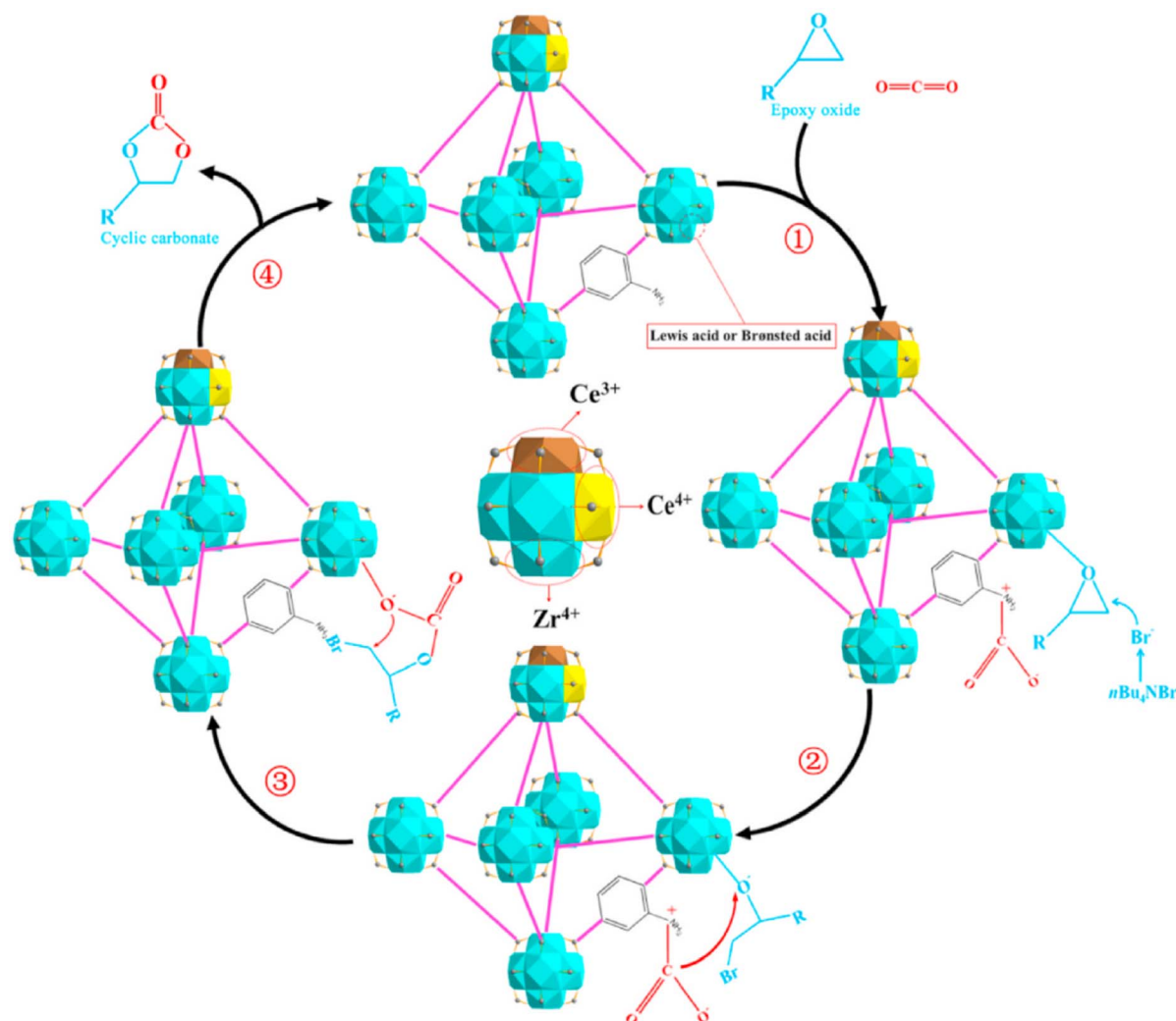
Fig. 16 Proposed mechanism for the cycloaddition of \text{CO}_2 and epoxides by a defective bimetallic \text{UiO}-66\text{-NH}_2(\text{Zr/Ce}) catalyst. (1) Through the catalyst, epoxy oxide is integrated with Lewis or Brønsted acid sites and is activated. Due to the presence of the -\text{NH}_2 group on the MOF, \text{CO}_2 is adsorbed and polarized; (2) the nucleophilic \text{Br}^- ion attacks the \beta carbon atom of epoxy to form the oxygen anion intermediate; (3) the intermediate interacts with \text{CO}_2 to create halogenated carbonate; (4) through internal cyclization, halogenated carbonate is converted into cyclic carbonate, while the catalyst is regenerated. Reproduced with permission from ref. 293, copyright 2021 Elsevier.
