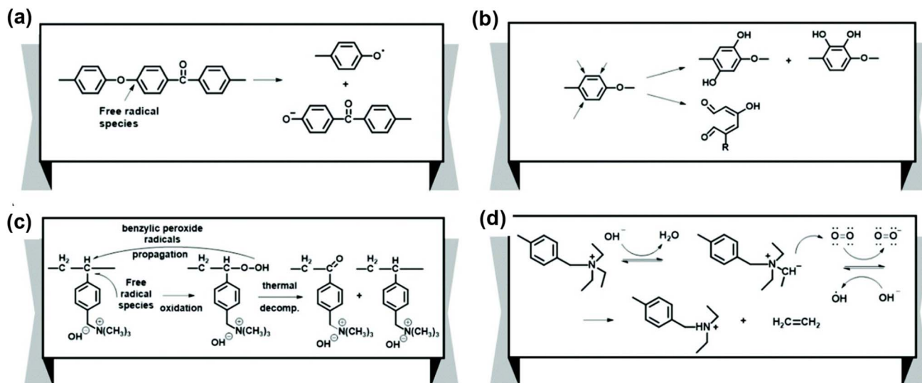
Fig. 11 Radical degradation pathways of AEMs: radicals attack both the polymer backbone and the functional groups. (a) Aryl ether polymer backbone degradation. (b) Phenyl group degradation by formation of phenolates. (c) Polymer backbone degradation of quaternized polystyrene. (d) Cationic group degradation. Adapted from Li et al. 163 with permission from the Royal Society of Chemistry.
