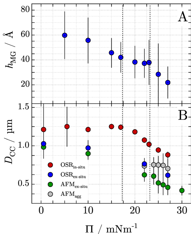
Fig. 7 (A) The first moment ( h_{\text{MG}} ) of the slabs j = 1, 2 that represent the parts of the MG that protrude into the air superphase above the apparent air/water interface ( z \geq 0 \text{ \AA} ), as calculated from the SLD profiles presented in Fig. 5. (B) Centre-to-centre distances ( D_{\text{cc}} ) of MG particles deduced with OSR at the air/water interface ( in situ ) and with AFM and OSR on Langmuir–Blodgett transferred samples ( ex situ ) as a function of lateral pressure \Pi .
