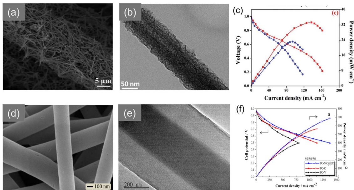
Fig. 12 (a) SEM and (b) TEM images of \text{Co}_3\text{O}_4@ \text{NiO} nanofibers. (c) Polarization of the DUFs with 50 \times 10^{-3} \text{ m} urea at RT. (a–c) adopted from ref. 234, Copyright© John Wiley and Sons- (2018). (d) SEM and (e) TEM images of \text{SiO}_2@ \text{C} core-shell nanofibers. (f) Polarization curves (I–V curves) and power density curves (I–P curves) of FC-V, FC-C, and FC- \text{SiO}_2@ \text{C} under different operating cells at 50^\circ \text{C} . (d–f) adopted from ref. 235, Copyright© Springer- (2018).
