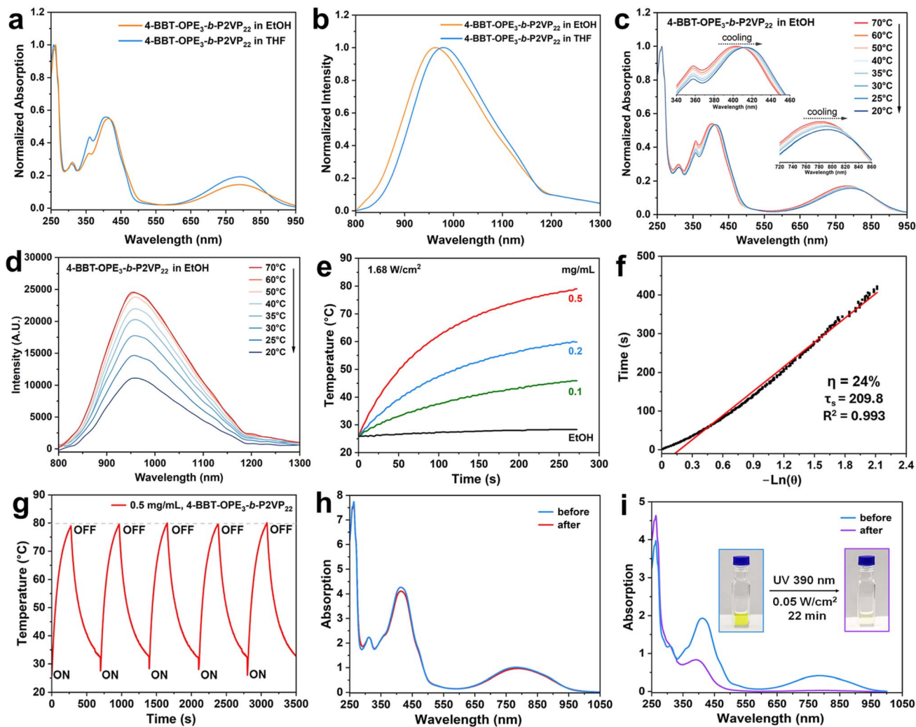
Fig. 3 NIR emission and photothermal activity of 4-BBT-OPE 3 -containing fiber-like micelles. (a) UV-vis-NIR absorption and (b) fluorescence spectra of 4-BBT-OPE 3 - b -P2VP 22 in ethanol and THF (0.05 mg mL -1 ). Temperature-dependent (c) UV-vis-NIR absorption and (d) fluorescence spectra of 4-BBT-OPE 3 - b -P2VP 22 in ethanol (0.05 mg mL -1 ). (e) Photothermal curves of ethanol and a micellar solution of 4-BBT-OPE 3 - b -P2VP 22 in ethanol with different concentrations (1.68 W cm -2 ). (f) Photothermal conversion efficiency of 4-BBT-OPE 3 - b -P2VP 22 (0.5 mg mL -1 and 1.68 W cm -2 ). (g) Photothermal curves of micellar solution (0.5 mg mL -1 ) of 4-BBT-OPE 3 - b -P2VP 22 in ethanol with five on/off cycles of irradiation (1.68 W cm -2 ). UV-vis-NIR absorption spectra of micellar solutions of 4-BBT-OPE 3 - b -P2VP 22 before and after (h) NIR (808 nm, 1.68 W cm -2 , and 0.5 mg mL -1 ) and (i) UV (390 nm, 0.05 W cm -2 , and 0.2 mg mL -1 ) irradiation for 22 min.
