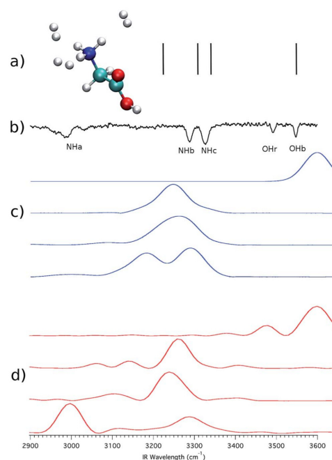
Fig. 2 Vibrational spectra for protonated glycine microsolvated by three H_2 molecules. Panel a): scaled harmonic estimates. Panel b): experimental spectrum; Panel c): QCT method results; Panel d): DC-SCIVR calculation. Reproduced from F. Gabas, G. Di Liberto, R. Conte and M. Ceotto, Chem. Sci. 2018, 9 , 7894–7901.
