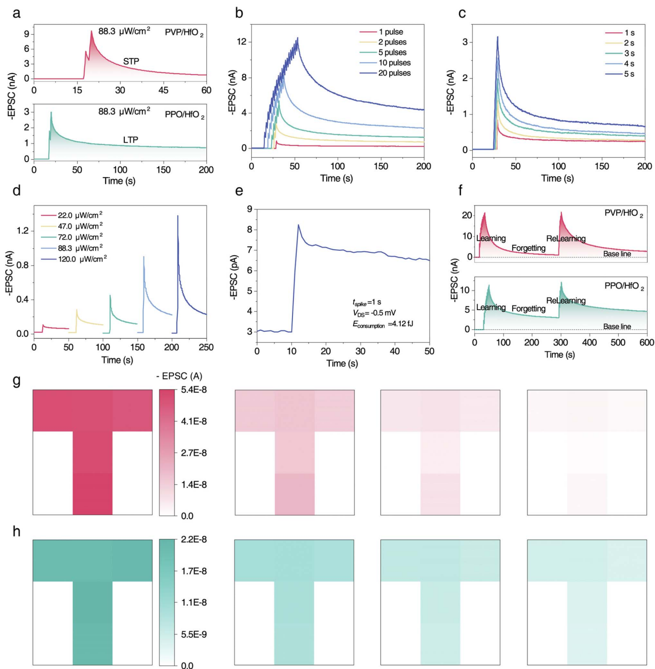
Fig. 3 (a) EPSC stimulated by two consecutive light pulses (365 nm, 88.3 μW cm -2 ) for PVP/HfO 2 -based and PPO/HfO 2 -based devices. The relationship between EPSC of the PPO/HfO 2 -based device and (b) light pulse number, (c) light pulse width, and (d) light pulse intensity. (e) The energy consumption of the PPO/HfO 2 -based device triggered by light pulses ( V_{\text{DS}} = -0.5 mV, t_{\text{spike}} = 1 s). (f) The learning–forgetting–relearning process for PVP/HfO 2 -based and PPO/HfO 2 -based devices. Image detection and memory of light-stimulated (g) PVP/HfO 2 -based and (h) PPO/HfO 2 -based devices with an input image of letter T.
