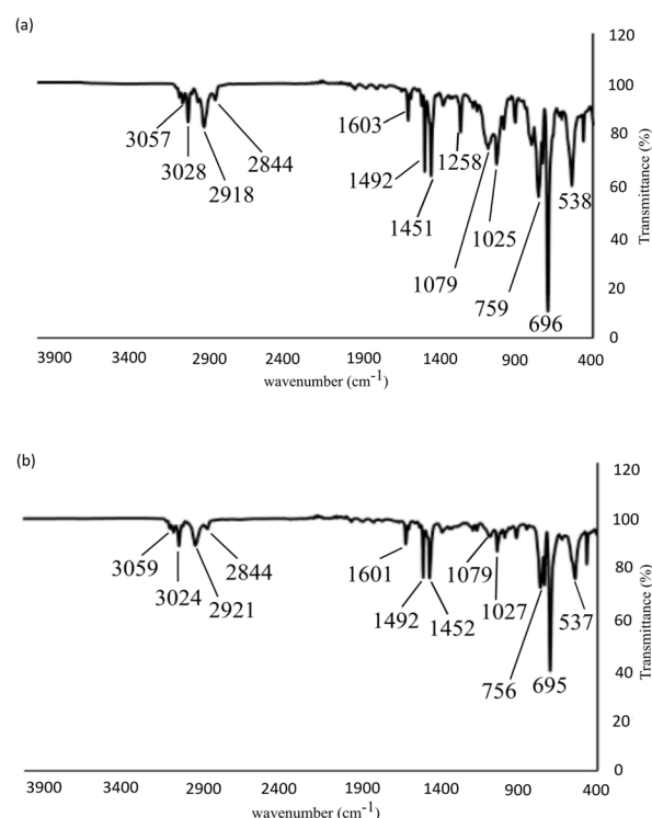
Fig. 4 (a) IR spectrum of syndiotactic polystyrene prepared using a 0.5 mol% catalytic loading of [\text{tBu}_2\text{Al}(6\text{-Me-py})_2] ( 1e ) and [\text{Ph}_3\text{C}][\text{B}(\text{C}_6\text{F}_5)_4] to generate cation 2e in situ at -15 °C. (b) IR spectra of atactic polystyrene prepared using a 0.5 mol% catalytic loading of [\text{Me}_2\text{Al}(6\text{-MeO-py})_2] ( 1c ) and [\text{Ph}_3\text{C}][\text{B}(\text{C}_6\text{F}_5)_4] to generate cation 2c in situ at 0 °C.
