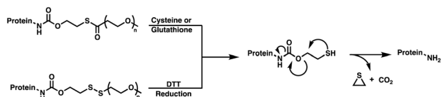
Fig. 7 Thioester (top) or disulfide (bottom) triggered mechanism of protein release for the \beta -mercaptopcarbamate traceless linkers.
