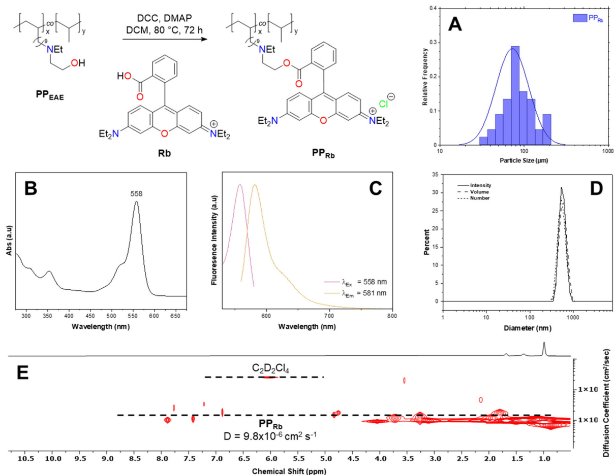
Fig. 1 Scheme: synthesis of PP Rb under Steglich esterification conditions, (A) solid particle size distribution histogram as determined by SEM (Fig. S9), (B) UV-Vis spectrum of PP Rb solution (0.5 mg mL -1 , chloroform), (C) fluorescence spectrum of PP Rb solution (0.5 mg mL -1 , chloroform), (D) DLS analysis of PP Rb solution (1 mg mL -1 , toluene), and (E) DOSY 1 H NMR spectrum (500 MHz, C 2 D 2 Cl 4 , 393 K) of PP Rb .
