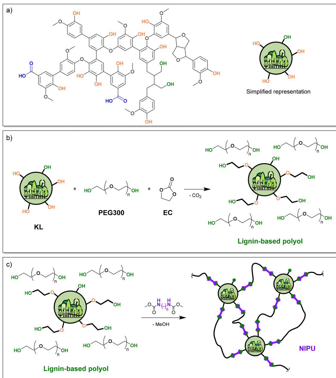
Fig. 1 (a) Representative structure of KL, (b) scheme of lignin-based polyol synthesis with EC and (c) scheme of NIPU synthesis from lignin-based polyol and HMDI.
