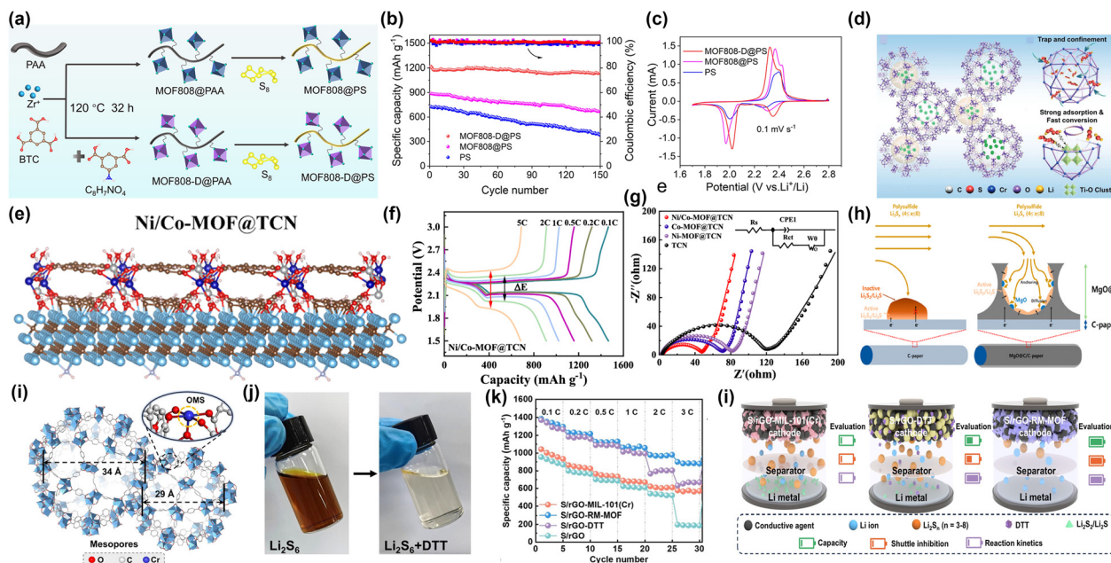
Fig. 17 (a) Schematic illustration of the synthesis routes for MOF808@PS and MOF808-D@PS sulfide composites. (b) Cycling performance of MOF808-D@PS, MOF808@PS, and pristine PS cathodes at 0.3 C. (c) Initial CV curves of the three cathodes recorded at 0.1 mV s -1 . Reproduced with permission from ref. 189 Copyright 2025 American Chemical Society. (d) Conceptual diagram of MOF-TOC frameworks acting as polar confinement matrices that trap polysulfides and catalyze their conversion. Reproduced with permission from ref. 252 Copyright 2023 John Wiley and Sons. (e) Synthesis schematic of the Ni/Co-MOF@TCN. (f) Galvanostatic charge–discharge profiles of Li–S cells using the Ni/Co-MOF@TCN/S cathode at various C-rates. (g) EIS of TCN, Ni-MOF@TCN, Co-MOF@TCN, and Ni/Co-MOF@TCN electrodes. Reproduced with permission from ref. 253 Copyright 2025 Elsevier. (h) Comparison of polysulfide transport on bare carbon paper (left) and MgO-coated carbon paper (right), where MgO provides strong anchoring sites that suppress shuttle effects and promote uniform Li 2 S x conversion. Reproduced with permission from ref. 254 Copyright 2023 American Chemical Society. (i) Structural representation of MIL-101(Cr) showing its large mesoporous cages (29–34 Å) and open metal sites. (j) Digital photographs showing the decolorization of Li 2 S 6 solution after addition of DTT, indicating strong polysulfide adsorption. (k) Rate capability of Li–S batteries using different cathodes between 0.1 C and 3 C. (l) Schematic summary of the polysulfide shuttle, reaction kinetics, and trapping behavior in Li–S cells employing the four cathode configurations. Reproduced with permission from ref. 255 Copyright 2025 Royal Society of Chemistry.
