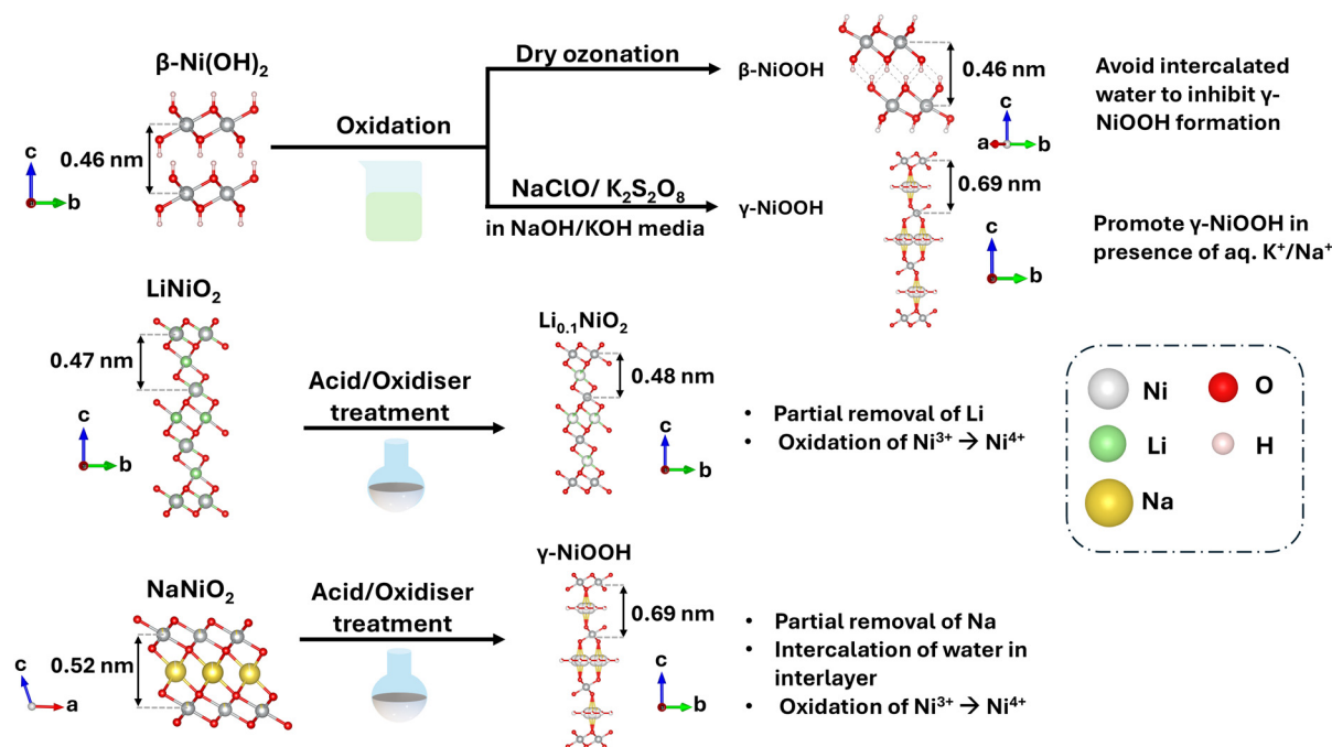
Fig. 5 Summary of basic synthesis routes adopted for the preparation of well-known high-valent nickel oxides ( \beta -NiOOH, 62 \gamma -NiOOH, 69 Li 0.1 NiO 2 101 ) using \beta -Ni(OH) 2 , 102 LiNiO 2 103 and NaNiO 2 104 as precursors. The crystal structures of the above-mentioned compounds were visualized using the VESTA software.
