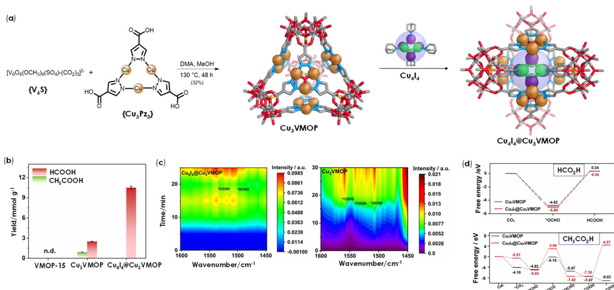
Fig. 4 (a) Sequential self-assembly of \text{Cu}_3\text{VMOP} and \text{Cu}_4\text{I}_4@\text{Cu}_3\text{VMOP} . (b) Comparison of yields and selectivity observed for the relevant catalysts during the \text{CO}_2 reduction reactions. (c) In situ DRIFTS spectra for detecting the reaction intermediates on \text{Cu}_4\text{I}_4@\text{Cu}_3\text{VMOP} and \text{Cu}_3\text{VMOP} . (d) Free-energy diagrams for \text{HCOOH} and \text{CH}_3\text{COOH} for \text{Cu}_3\text{VMOP} and \text{Cu}_4\text{I}_4@\text{Cu}_3\text{VMOP} . Parts (b–d) adapted from ref. 56, https://doi.org/10.1002/anie.202423018 . Copyright 2025, Wiley-VCH.
