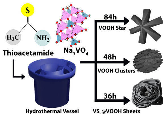
Fig. 2 Schematic representation of the synthetic procedure of vanadyd hydroxide stars.
