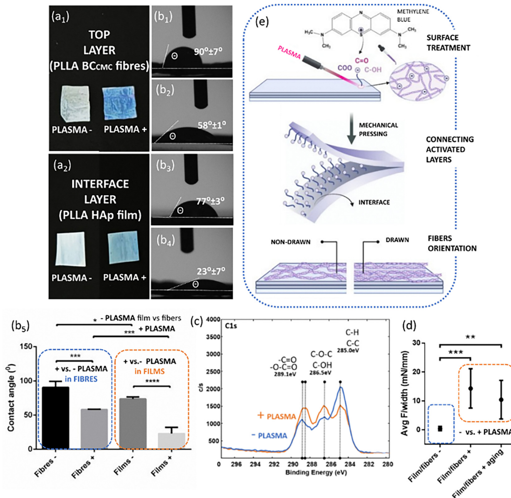
Fig. 2 Surfaces and interface in two-layered PLLA structures. Methylene blue (MB) staining of PLLA BC CMC fibres and PLLA HAp smooth films with and without plasma treatment (a 1 –a 2 ); water contact angles at the surface of films and fibres and statistically relevant differences induced by nanostructuring and plasma (b 1 –b 5 ); XPS spectra of PLLA surface before and after plasma treatment (c); adhesion between layers following plasma activation, and plasma stability (aging) (d), toward two-layered structure: surface activation, connecting activated layers and fibers orientation at the top (e), *, **, *** and **** indicate p < 0.05 , p < 0.005 , p < 0.001 and p < 0.0001 , respectively.
