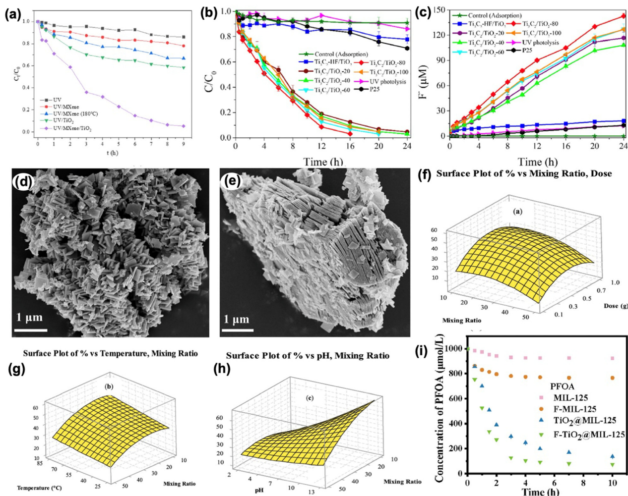
Fig. 14 (a) Photocatalytic degradation of PFOA under different systems: UV alone, MXene, hydrothermally treated MXene ( 180^\circ\text{C} ), \text{TiO}_2 , and MXene/ \text{TiO}_2 composite. The MXene/ \text{TiO}_2 composite achieved the highest degradation (94.6%) due to enhanced light absorption and improved electron-hole separation, while UV alone showed minimal PFOA removal (13.96%). Reproduced from ref. 282 with permission from Elsevier BV, copyright 2025; photocatalytic degradation of PFOA using \text{Ti}_3\text{C}_2/\text{TiO}_2 -based catalysts: (b) PFOA removal under adsorption, UV photolysis, \text{Ti}_3\text{C}_2\text{-HF}/\text{TiO}_2 , P25, and \text{Ti}_3\text{C}_2/\text{TiO}_2\text{-80} , (c) fluoride ion ( \text{F}^- ) generation and defluorination efficiency for the same systems, (d) \text{TiO}_2 distribution within \text{Ti}_3\text{C}_2\text{-DES} showing intercalation into interlayers, (e) \text{TiO}_2 growth on the \text{Ti}_3\text{C}_2\text{-HF} surface for comparison. The intercalation strategy ( \text{Ti}_3\text{C}_2/\text{TiO}_2\text{-80} ) significantly enhances both PFOA degradation ( >99.9\% ) and defluorination (49%) compared to conventional \text{TiO}_2 systems. Reproduced from ref. 283 with permission from Elsevier BV, copyright 2020; three-dimensional RS (response surface) diagrams illustrating the optimal operating conditions for maximum treatment efficiency: (f) effect of catalyst dosage (0.5–0.7 g) and zeolite mixing ratio ( \sim 10\% ) on efficiency; (g) influence of the zeolite ratio ( \sim 10\% ) and reaction temperature (up to 85^\circ\text{C} ); (h) effect of the zeolite ratio ( \sim 10\% ) and pH (up to 13). The diagrams indicate that treatment efficiency improves with decreasing zeolite ratio, increasing temperature, and higher pH under the specified conditions. Reproduced from ref. 284 with permission from Elsevier BV, copyright 2024; (i) PFOA degradation by MIL-125, F-MIL-125, \text{TiO}_2\text{@MIL-125} , and F- \text{TiO}_2\text{@MIL-125} showed fastest kinetics for F- \text{TiO}_2\text{@MIL-125} with K_{\text{app}} = 1.221 \times 10^{-4} \text{ s}^{-1} , higher than that of other \text{TiO}_2 -based catalysts, while only \text{TiO}_2\text{@MIL-125} and F- \text{TiO}_2\text{@MIL-125} continued significant degradation after 2 h. Reproduced from ref. 66 with permission from Elsevier BV, copyright 2022. 66
