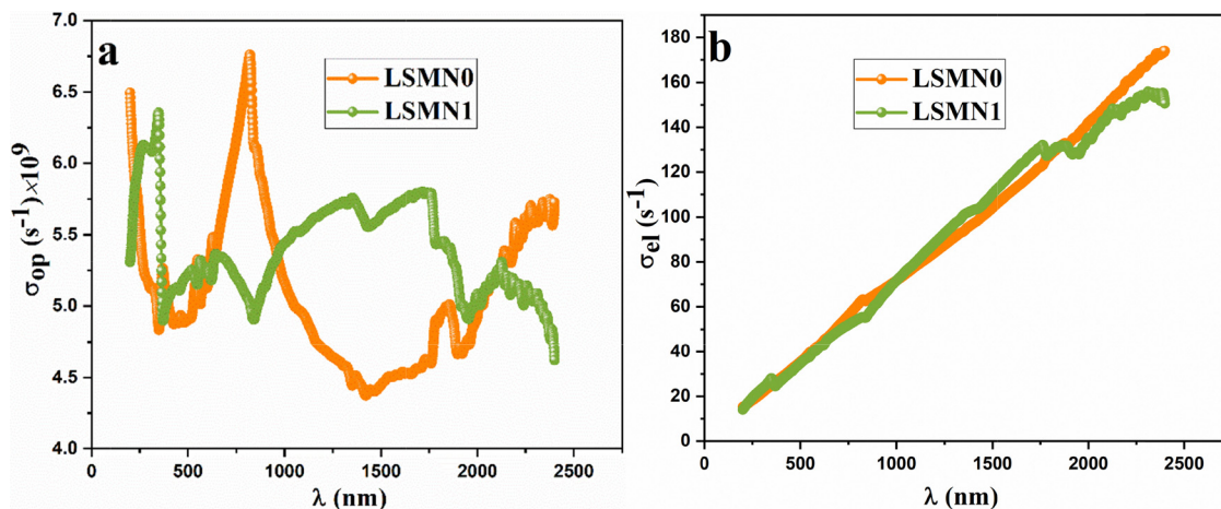
Fig. 12 (a) Spectral variation of optical conductivity \sigma_{op}(\lambda) . (b) Spectral variation of electrical conductivity \sigma_{el}(\lambda) for LSMN0 and LSMN1.
