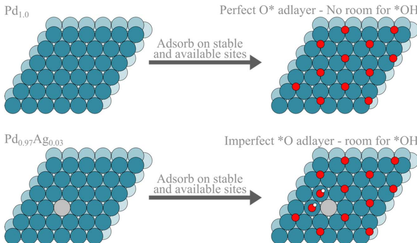
Fig. 4 Coverage of adsorbed species using extended blocking rules for Pd(111) (top row) and Pd(111) with a single Ag atom (bottom row). The presence of ^*\text{OH} species in Pd(111) with a single Ag atom improves the ORR activity by one order of magnitude.
