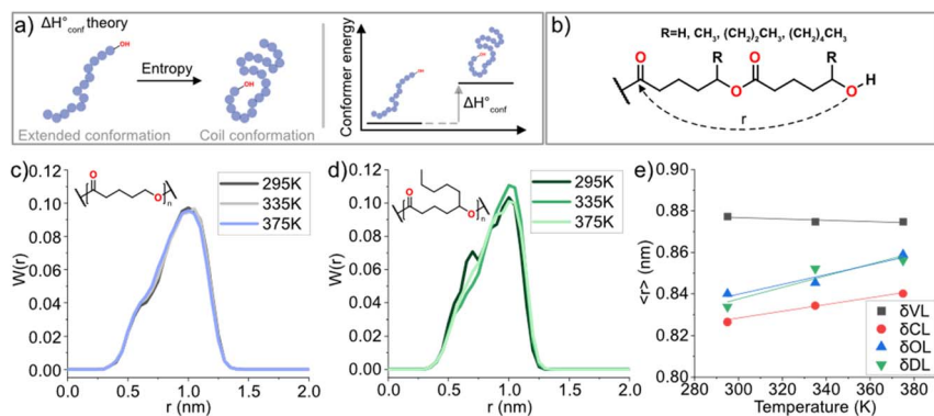
Fig. 6 Schematic representation of (a) the origins of \Delta H_{\text{conf}}^\circ and (b) the intramolecular distance used as proxy for polymer conformation. Conformational probability density distribution for r at different temperatures for (c) P \delta VL and (d) P \delta DL. (e) Average distance \langle r \rangle at different temperatures for polymers dissolved in toluene.
