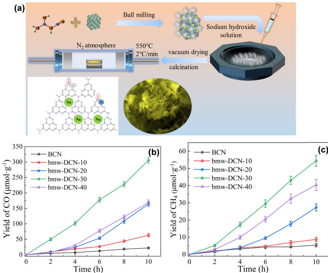
Fig. 22 (a) Diagrammatic illustration of the synthesis of Na-doped flaky g\text{-C}_3\text{N}_4 with N-defects, (b) CO and (c) \text{CH}_4 evolution rates of BCN and bmw-DCN- x . Reproduced with permission from ref. 151. Copyright 2021, Elsevier.
