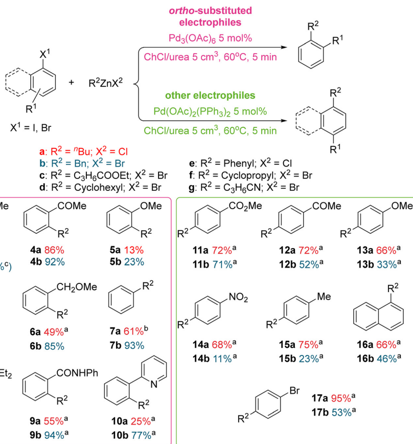
Scheme 4 Final substrate scope results for both ortho -coordinating group and other substituted iodoarenes. \text{R}^2\text{ZnX}^2 (1 mmol) in 2 cm 3 dry THF was added slowly to ArI (0.5 mmol) and Pd pre-catalyst (5 mol% Pd) in 5 cm 3 “wet” ChCl/urea at 60 °C. The reaction was stirred for 5 min at 1000 rpm before workup. GC yields determined by gas chromatography. a 1.5 mmol of \text{R}^2\text{ZnX}^2 used. b 2 mol% Pd pre-catalyst used. c \text{X}^1 = \text{Br} . d 2 mmol \text{R}^2\text{ZnBr} used.
