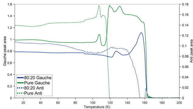
Fig. 6 Peak area of the gauche and anti conformer CH 2 twist mode measured over temperature for the 0.2 K min -1 ramping rate of the pure (green) and mixed ices (blue).
