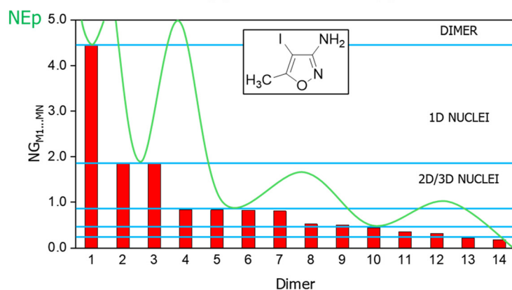
Fig. 6 Retrocrystallization scheme (top) and the normalized energies showing the crystallization process of 3-amino-4-iodo-5-methisoxazole (bottom).
