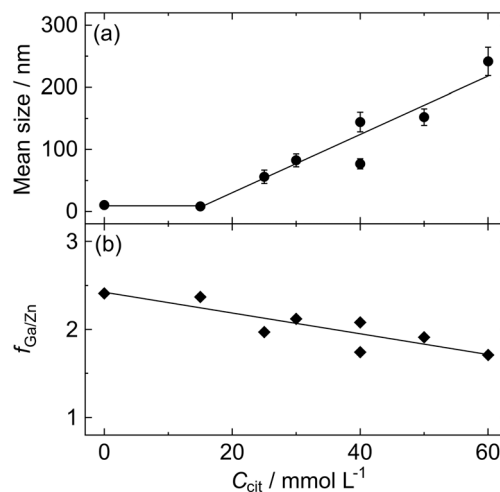
Fig. 4 Effect of the \text{Na}_3\text{-Cit} concentration ( C_{\text{cit}} ) on (a) the mean size and (b) atomic \text{Ga/Zn} ratio ( f_{\text{Ga/Zn}} ) of the ZGO particles synthesized under the conditions at C_{\text{Ga}}/C_{\text{Zn}} = 2.57 and 150 °C for 24 h.
