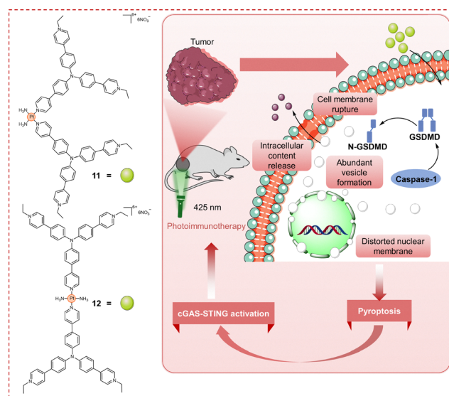
Fig. 16 Chemical structures and mechanism of action for complexes 11 and 12 . Upon photoactivation, these agents cause damage to DNA and the nuclear envelope, inducing pyroptotic cell death and activating the cGAS-STING pathway (cyclic GMP–AMP synthase–stimulator of interferon genes), which collectively stimulates an anticancer immune response in vitro and in vivo .
