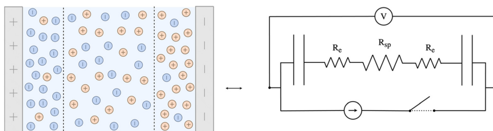
Fig. 6 Circuit-EDL analogy, represented by two capacitors in series with their internal resistance R_{\text{e}} , in series with the channel resistance R_{\text{sp}} .
