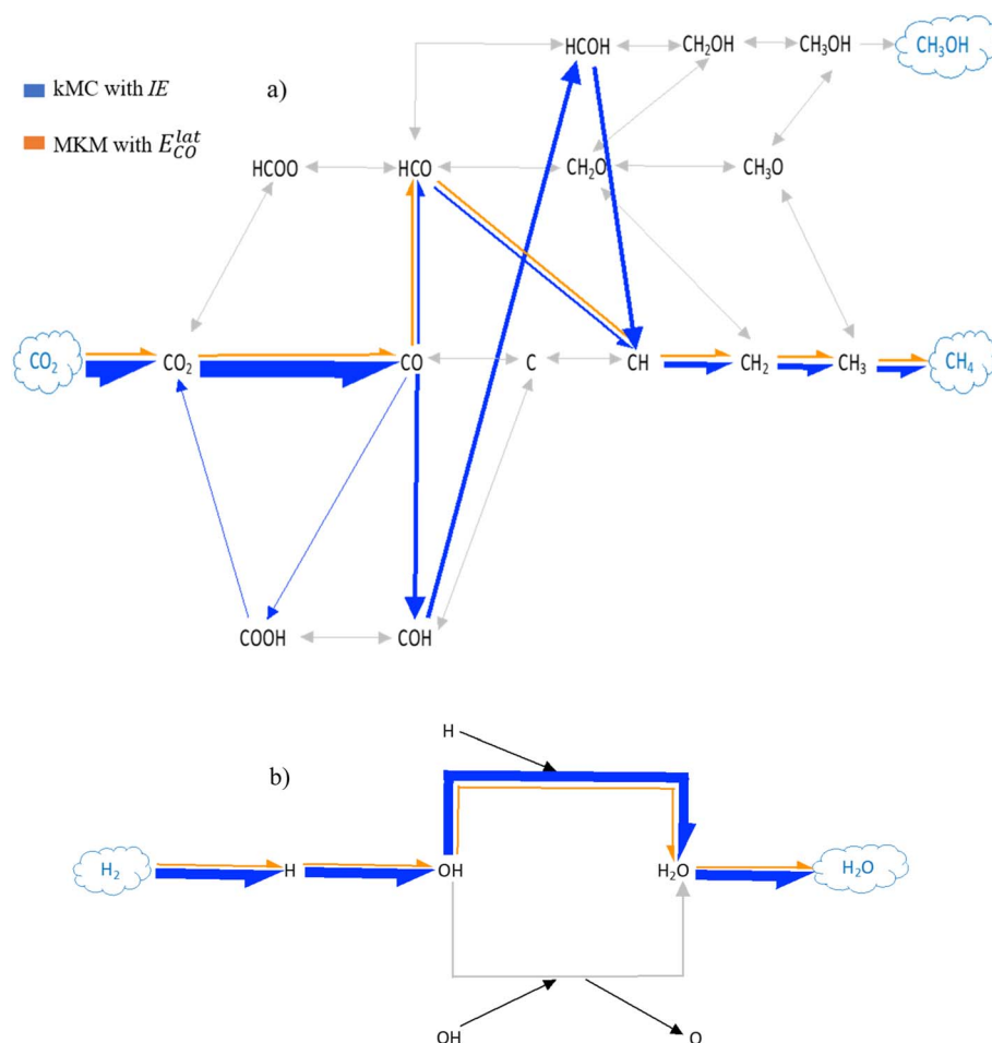
Fig. 4 Schematic representation of the most plausible mechanism for (a) CO 2 hydrogenation and (b) H 2(g) transformation into H 2O(g) over Ni(111) at T = 673.15 K and P = 10 bar with a CO 2 : H 2 molar ratio of 1 : 4 under condition (II), in which CO and CH 2 O are not allowed to desorb. Coloured arrows refer to produced events while grey arrows are for events that do not occur. The arrow's thickness symbolizes the net event frequency of each elementary process. MkM with coverage-dependent lateral potential ( E_{CO}^{lat} ) and kMC results with interaction energies (IE) in orange and blue, respectively. For details on the calculations for the arrow's thickness the reader is referred to Section S5.†
