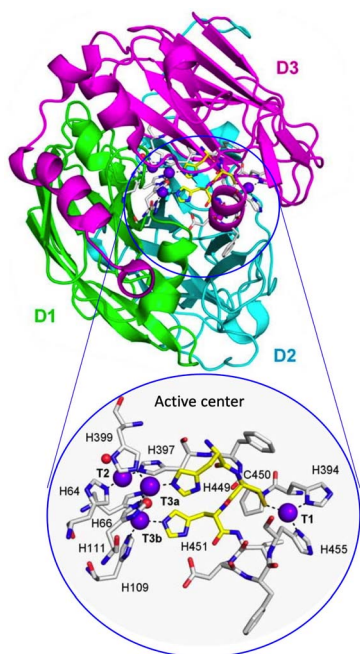
Fig. 2 Ribbon diagram of laccase from Trametes versicolor (PDB ID: 1GYC). The bottom part is a representation model of the Cu cluster in the active site. This picture was produced using data reported in ref.81 and 82.
