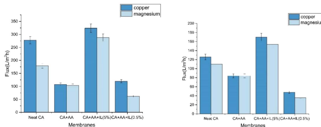
(e) NF performance of membranes at a pressure of 6 bar at pH 4
