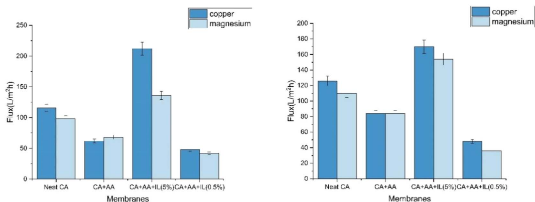
(c) NF performance of membranes at a pressure of 4 bar at pH 4
