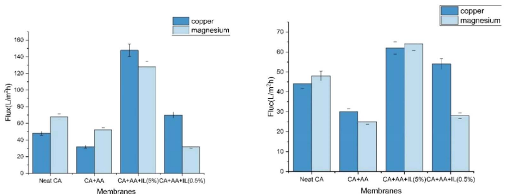
(b) NF performance of membranes at a pressure of 2 bar at pH 7
